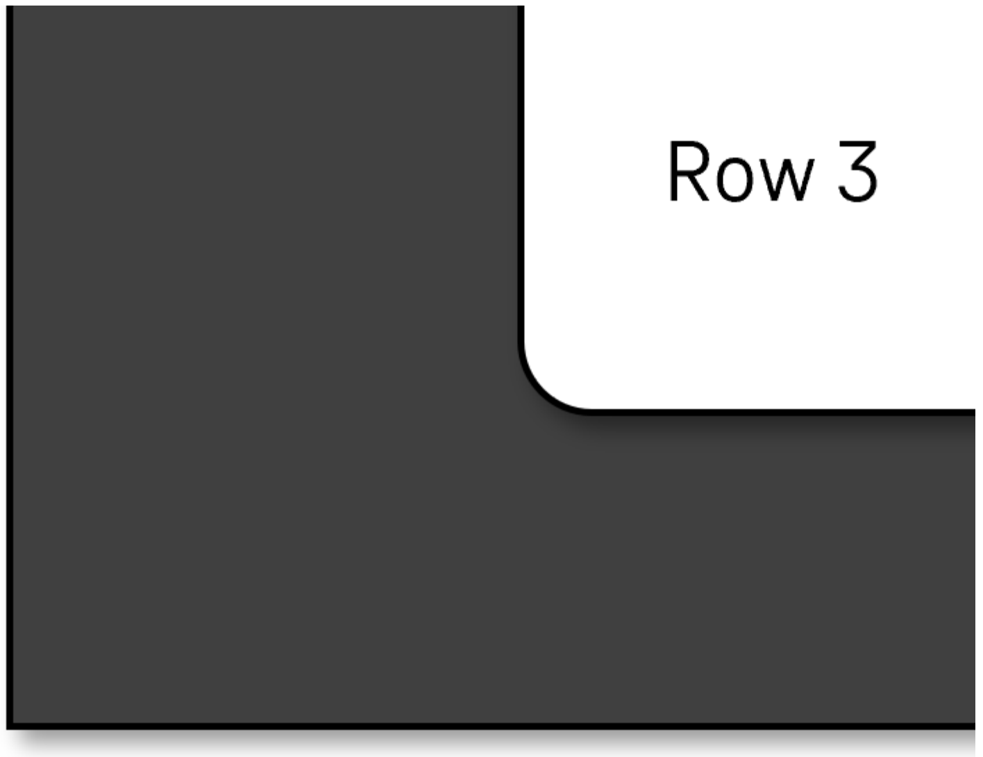
Figure 27: Modal dialog
