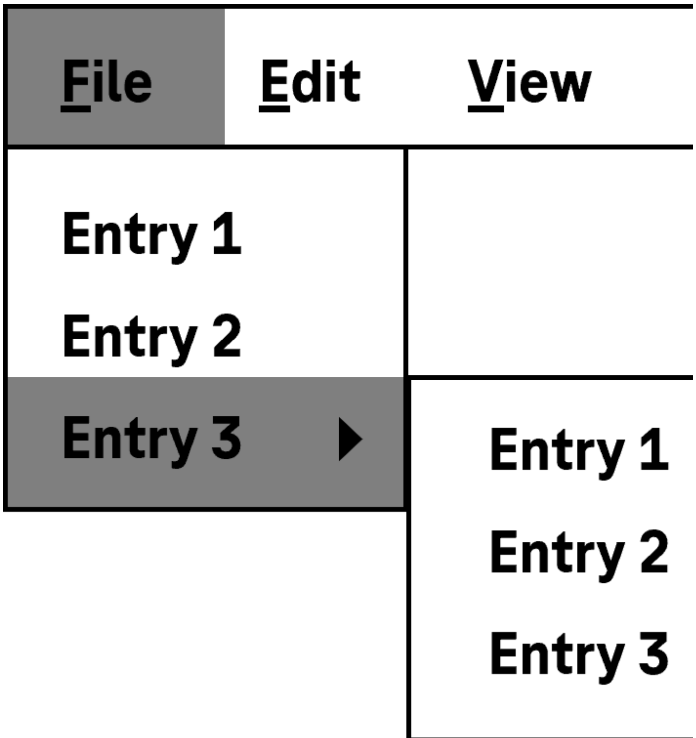
Figure 35: Application menu
