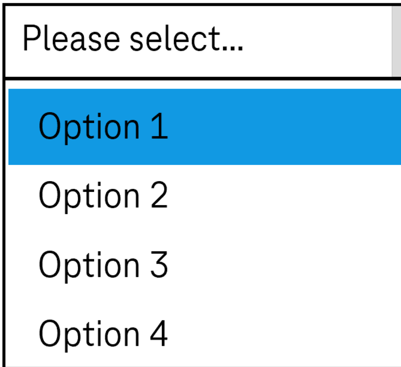
Figure 49: Drop-down list
