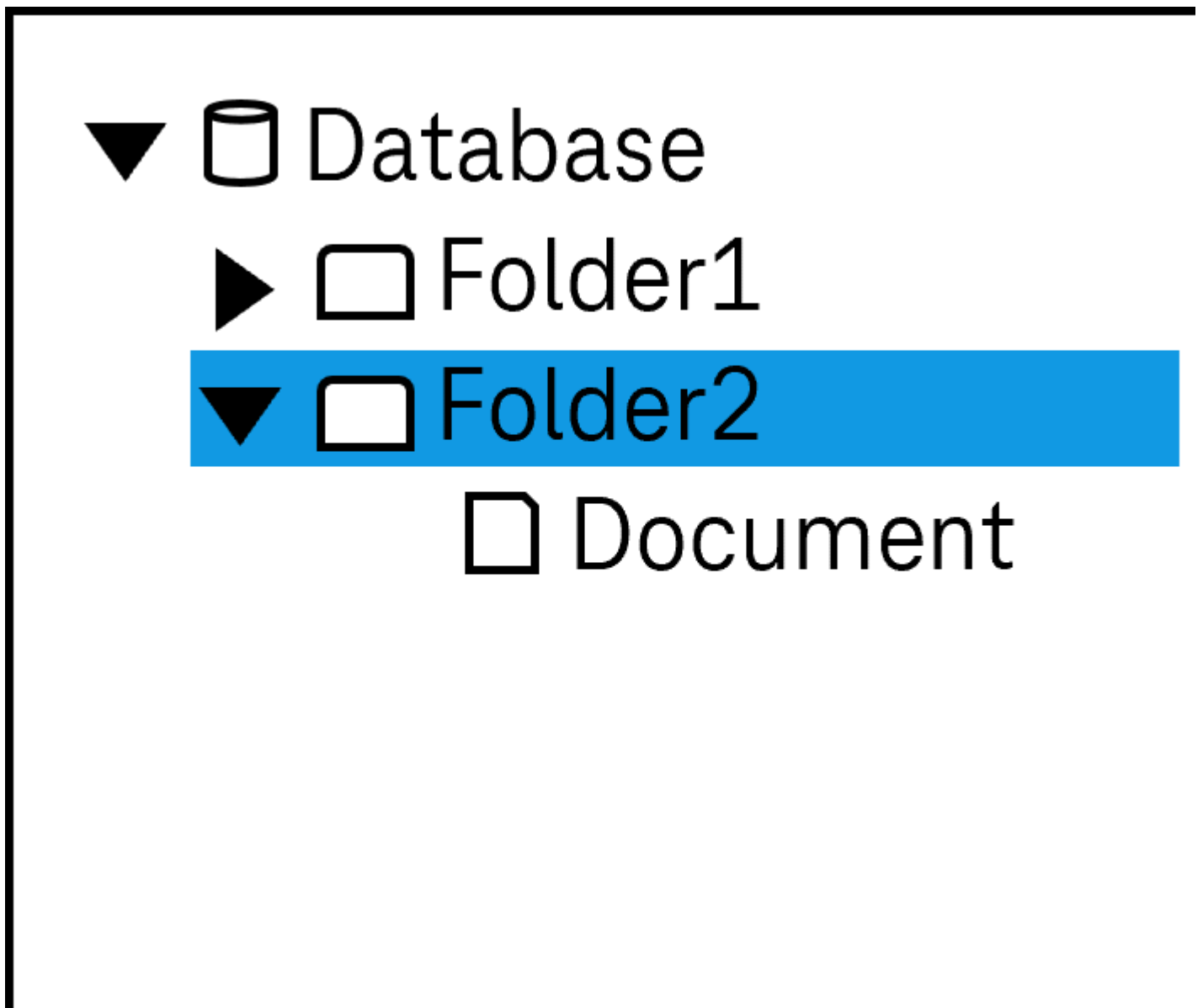
Figure 46: Tree structure
