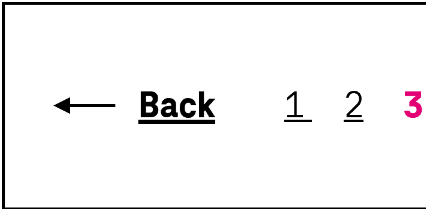
Figure 54: Pagination
