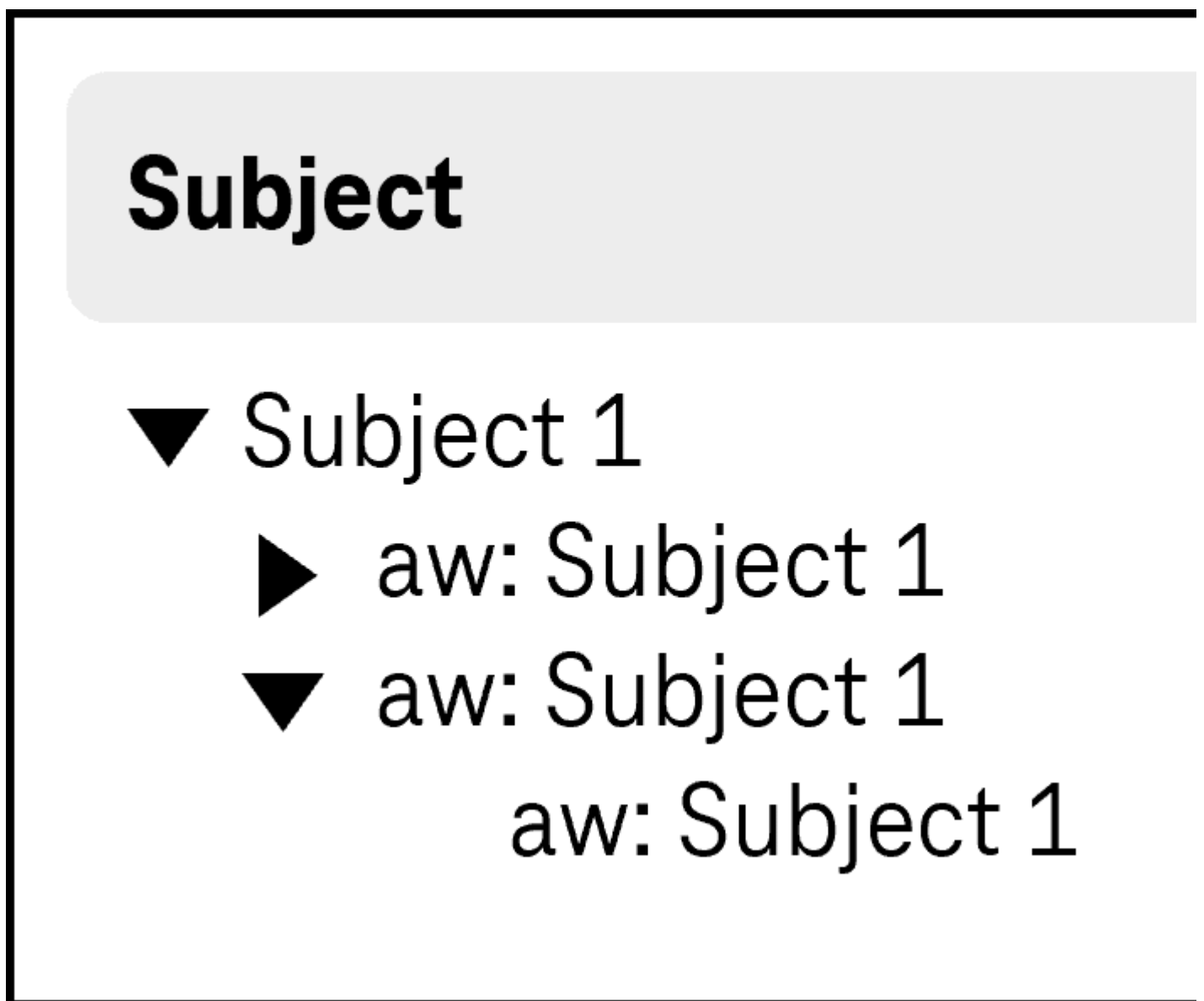
Figure 24: Hierarchical table
